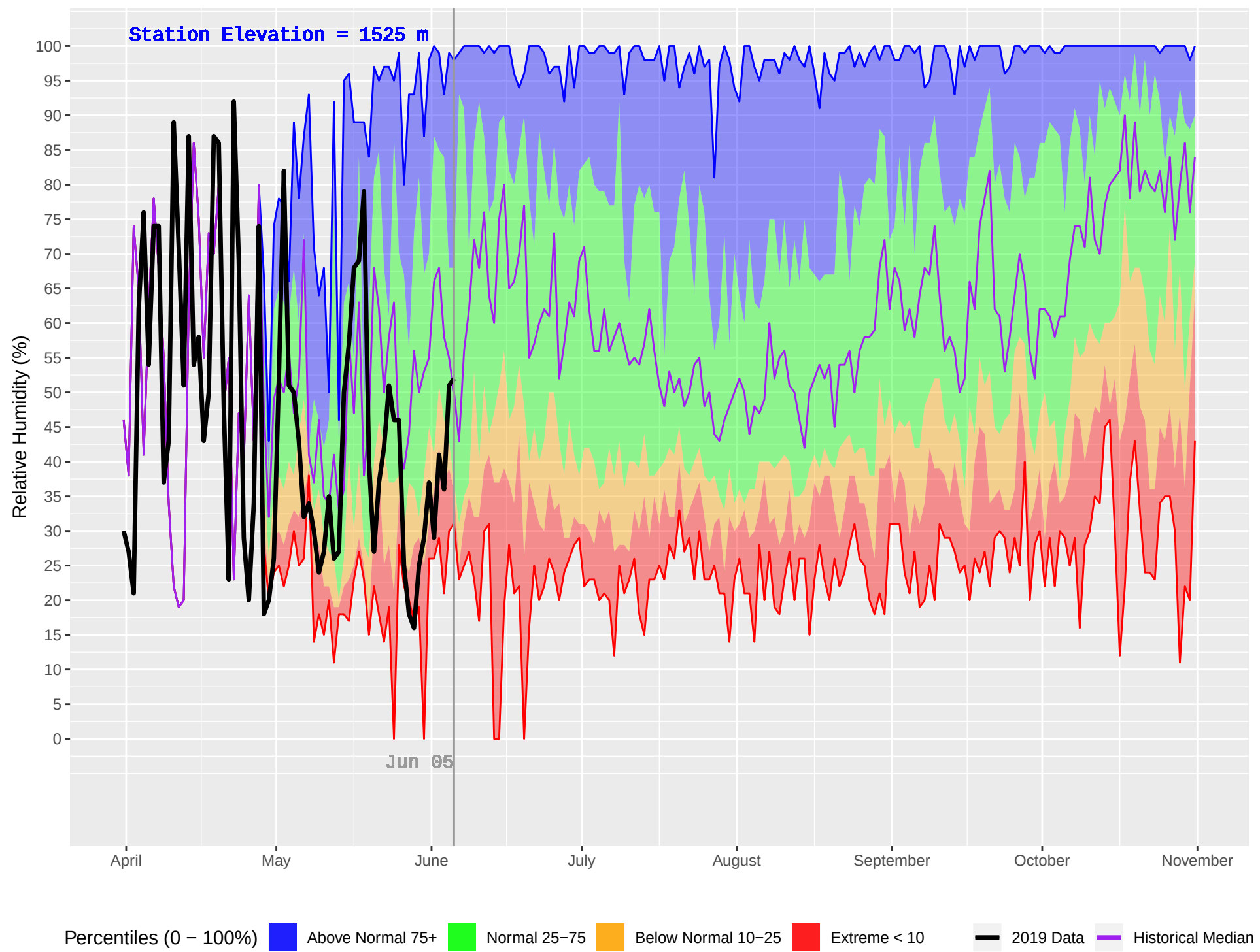
HARBOUR LAKE (250) : Historical (1989–2018) and Current (2019) Daily Relative Humidity
