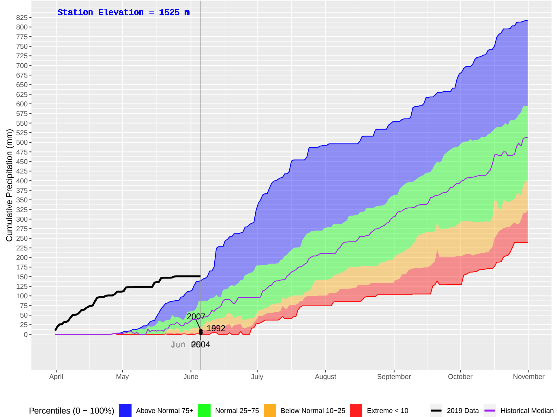
HARBOUR LAKE (250) : Historical (1989–2018), Current (2019) Daily Cumulative Precipitation
